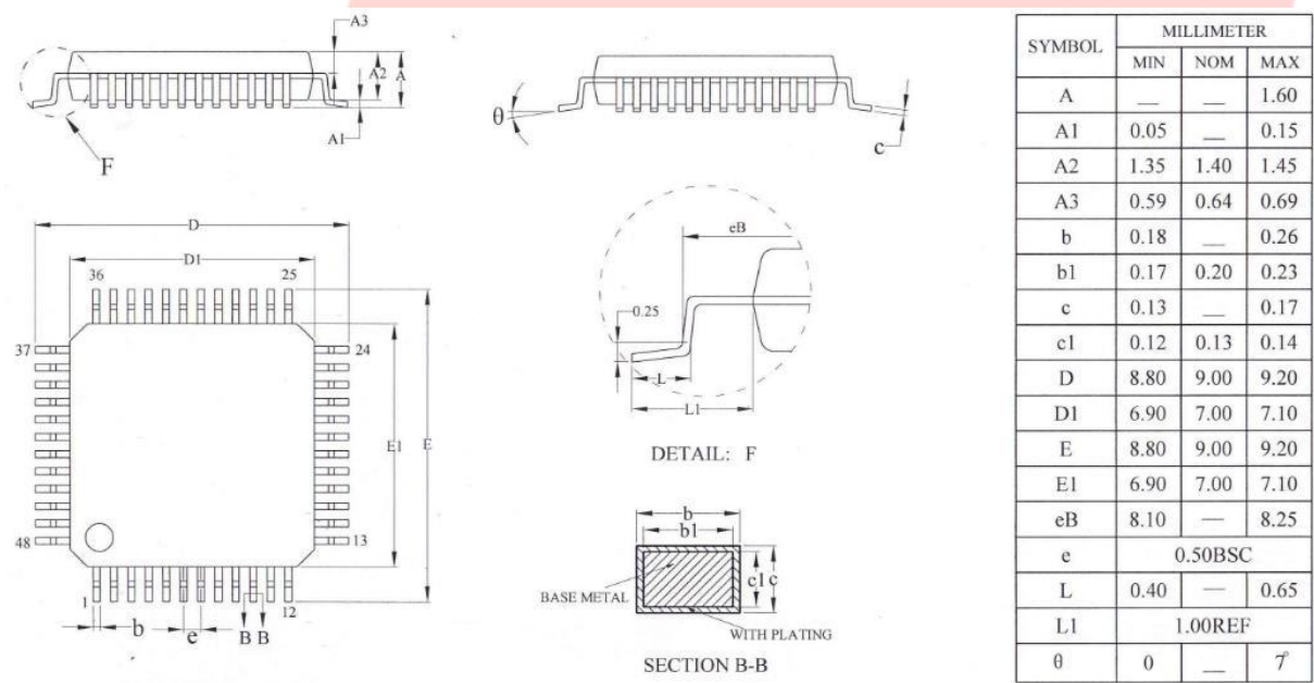
Figure 3-1. AC6351D_LQFP48 Package
