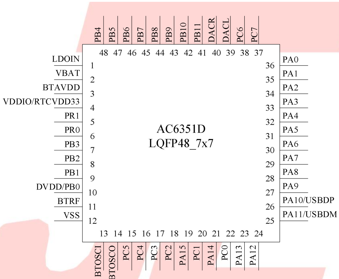
Figure 1-1 AC6351D_LQFP48 Package Diagram
