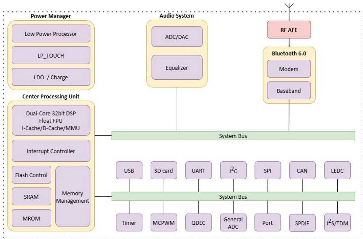
Figure 1-1 JL7094A Block Diagram
