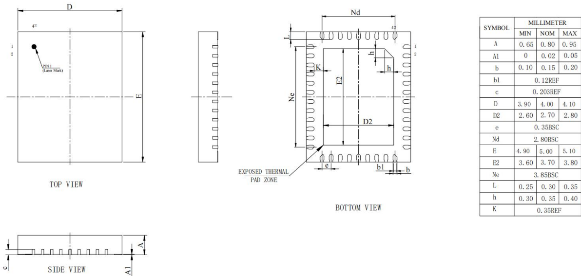
Figure 4-1 JL7094A Package
