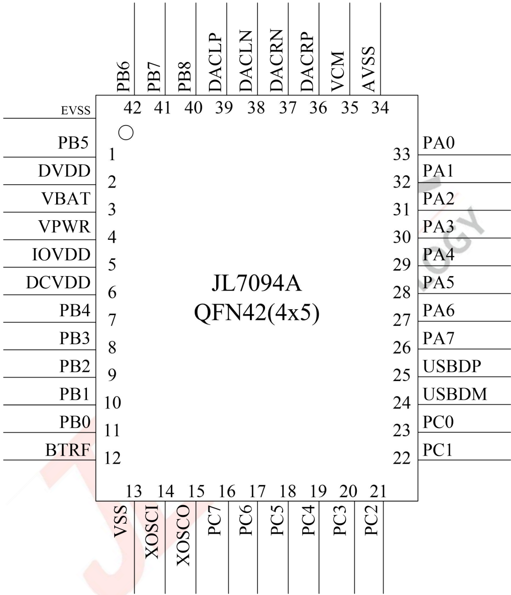
Figure 2-1 JL7094A Pin Assignment
