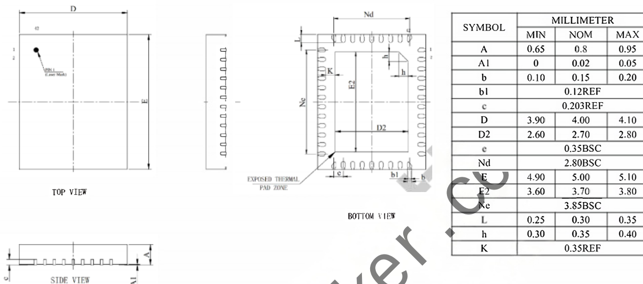
Figure 4-1 AC7074A Package
