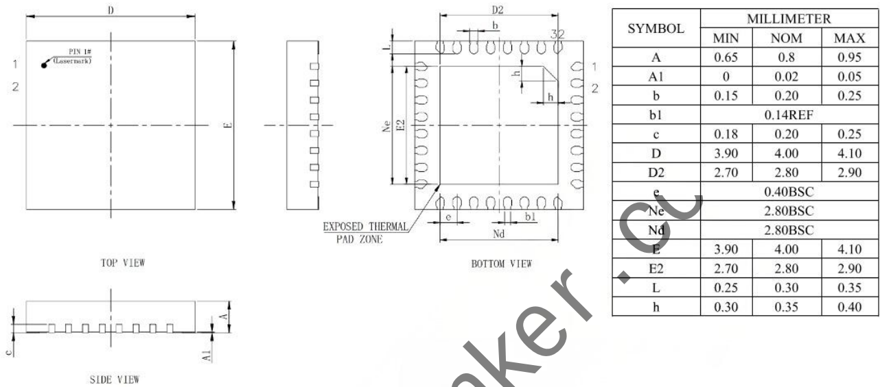
Figure 4-1 AC7076A Package
