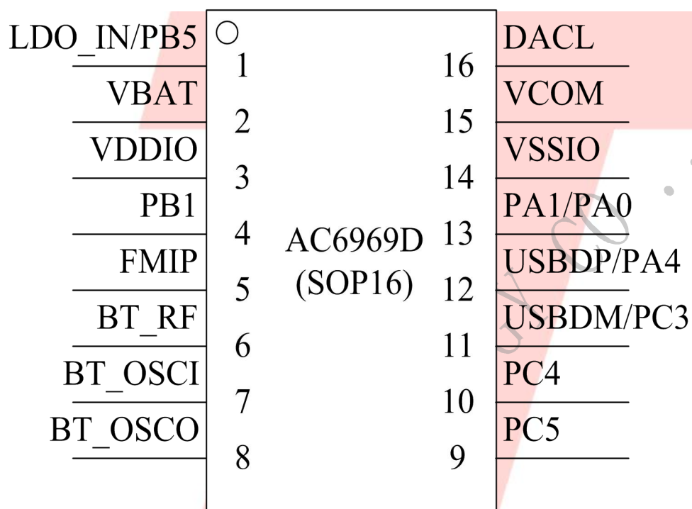
Figure 1-1 AC6969D Package Diagram
