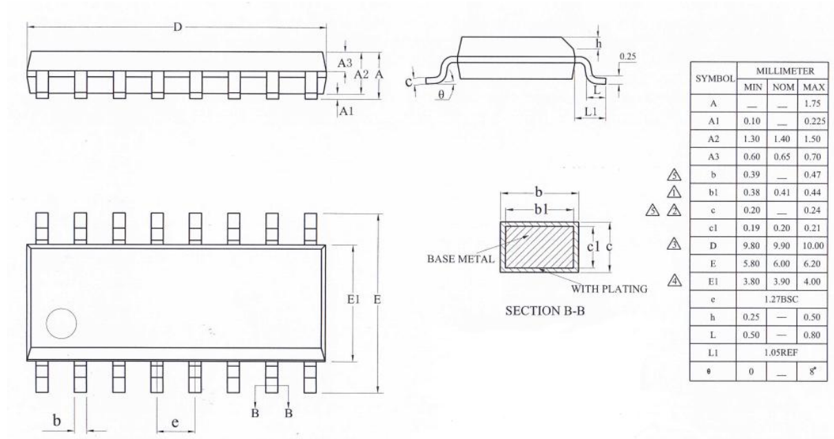
Figure 4-1 AC7069A Package
