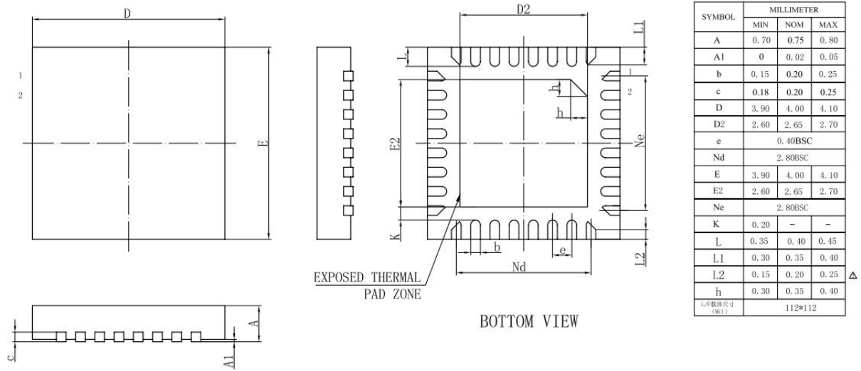
Figure 4-1 AC7066D Package
