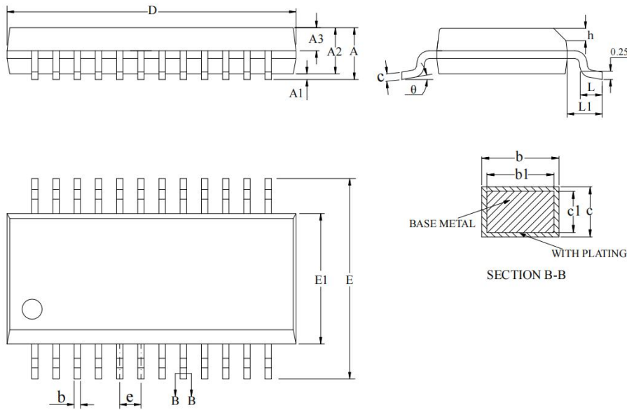
Figure 4-1 AC7065E Package
