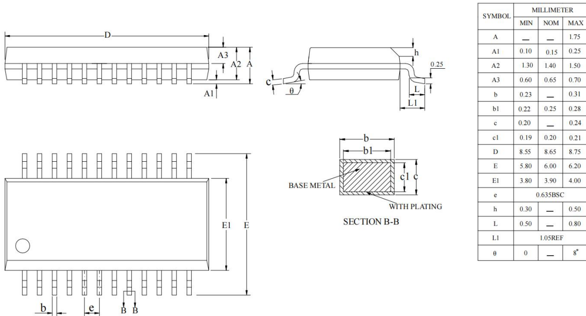
Figure 4-1 AC7065D Package
