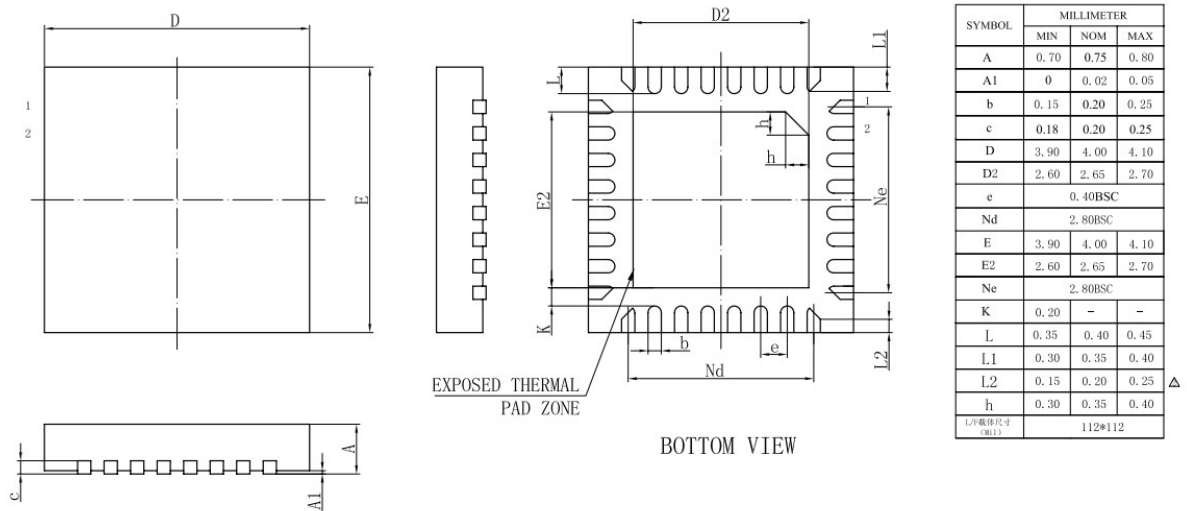
Figure 3-1. AD156A_QFN32 Package
