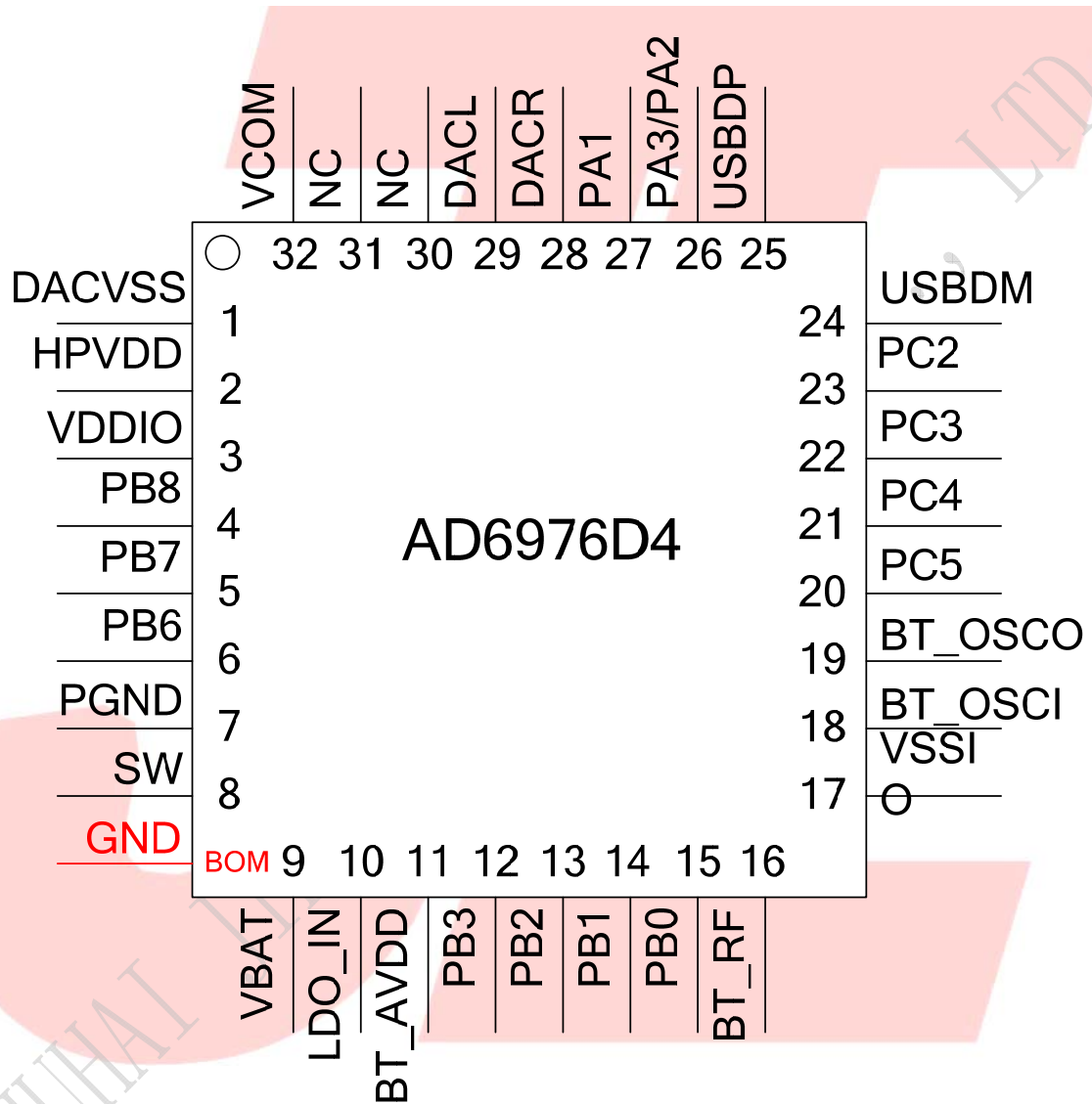
Figure 1-1 AD6976D4 Package Diagram
