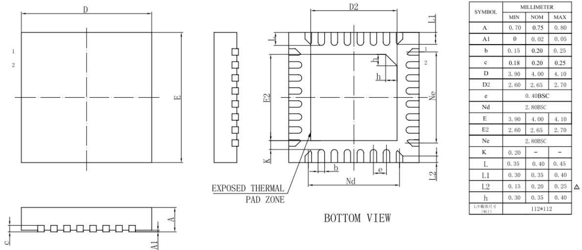
Figure 3-1 AD6976D4 Package
