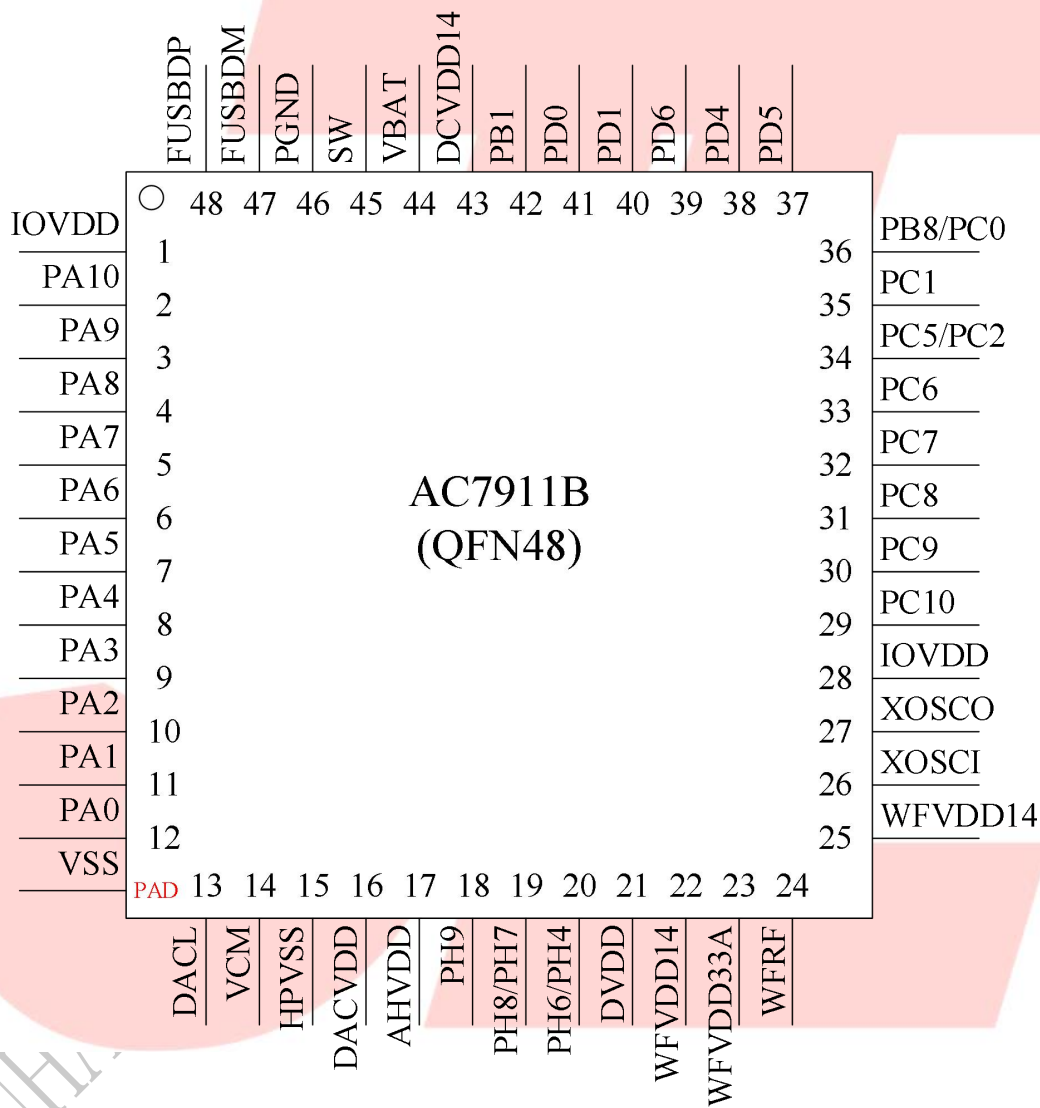
Figure 1-1 AC7911B_QFN48 Package Diagram
