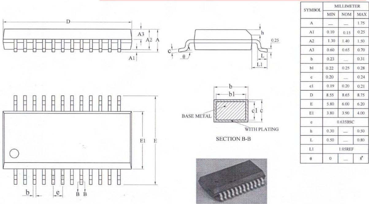
Figure 3-1. AC6965A Package
