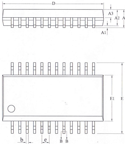
Figure 3-1. AD153A_QSOP24 Package
